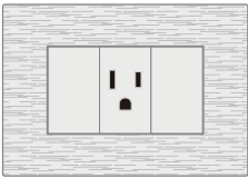
VS105 American socket 15A 250V~
