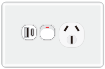
KS313-A+C 10A horizontal single power point with Type-C+USB 5V 2A KS313-A+C-D 10A horizontal single power point with Type-C+USB 20W PD
