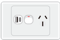
AS313-A+C 10A horizontal single power point with Type-C+USB 5V 2A AS313-A+C-D 10A horizontal single power point with Type-C+USB 20W PD
