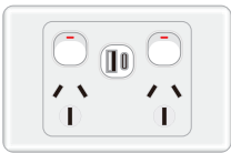
AS315-A+C 10A horizontal double power points with Type-C+USB 5V 2A AS315-A+C-D 10A horizontal double power points with Type-C+USB 20W PD AS318-A+C-D 10A horizontal double power points DP with Type-C+USB 20W PD
