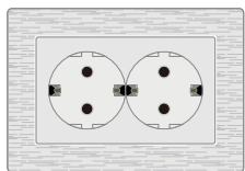
G6-129 Double german socket 16A 250V~ (With shutter)
